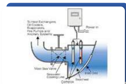
Antifouling Anode & Cathodic protection
